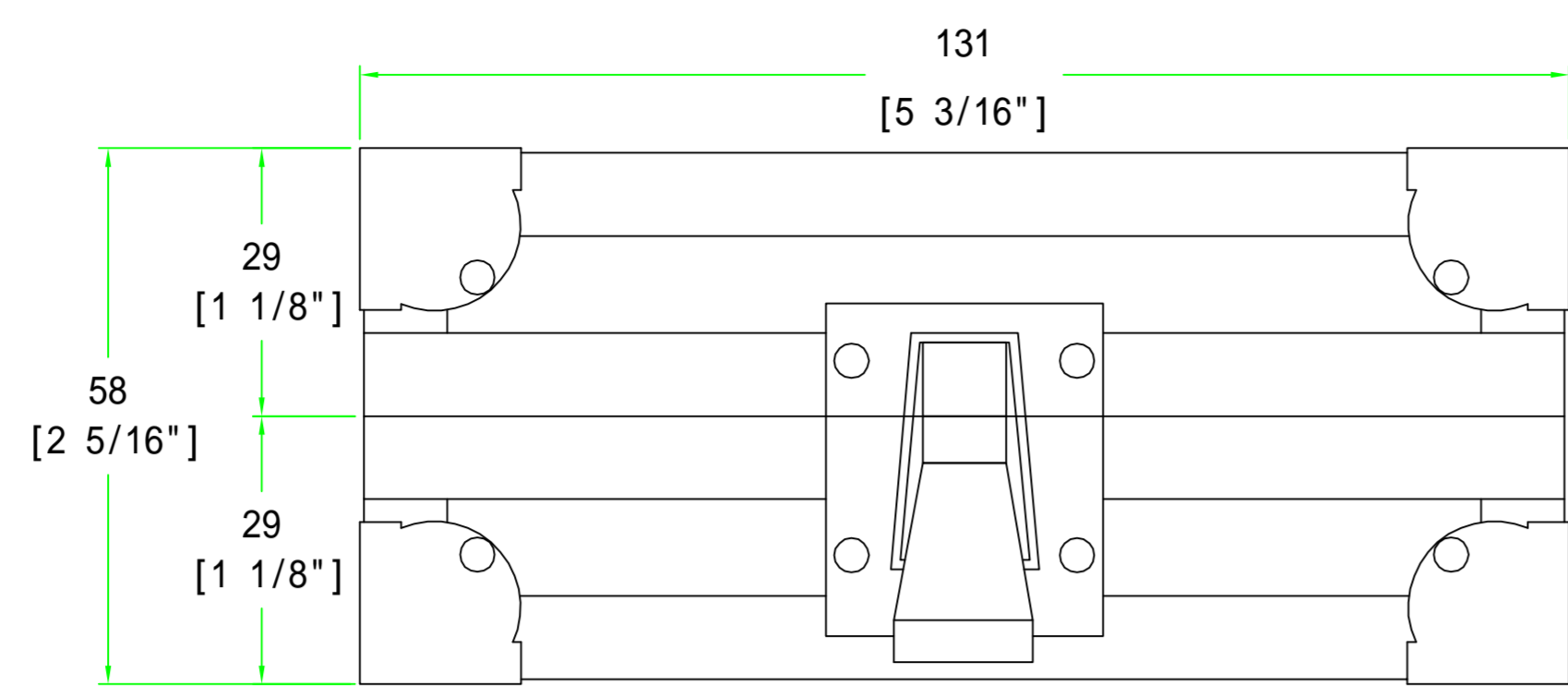
FRONT VIEW
