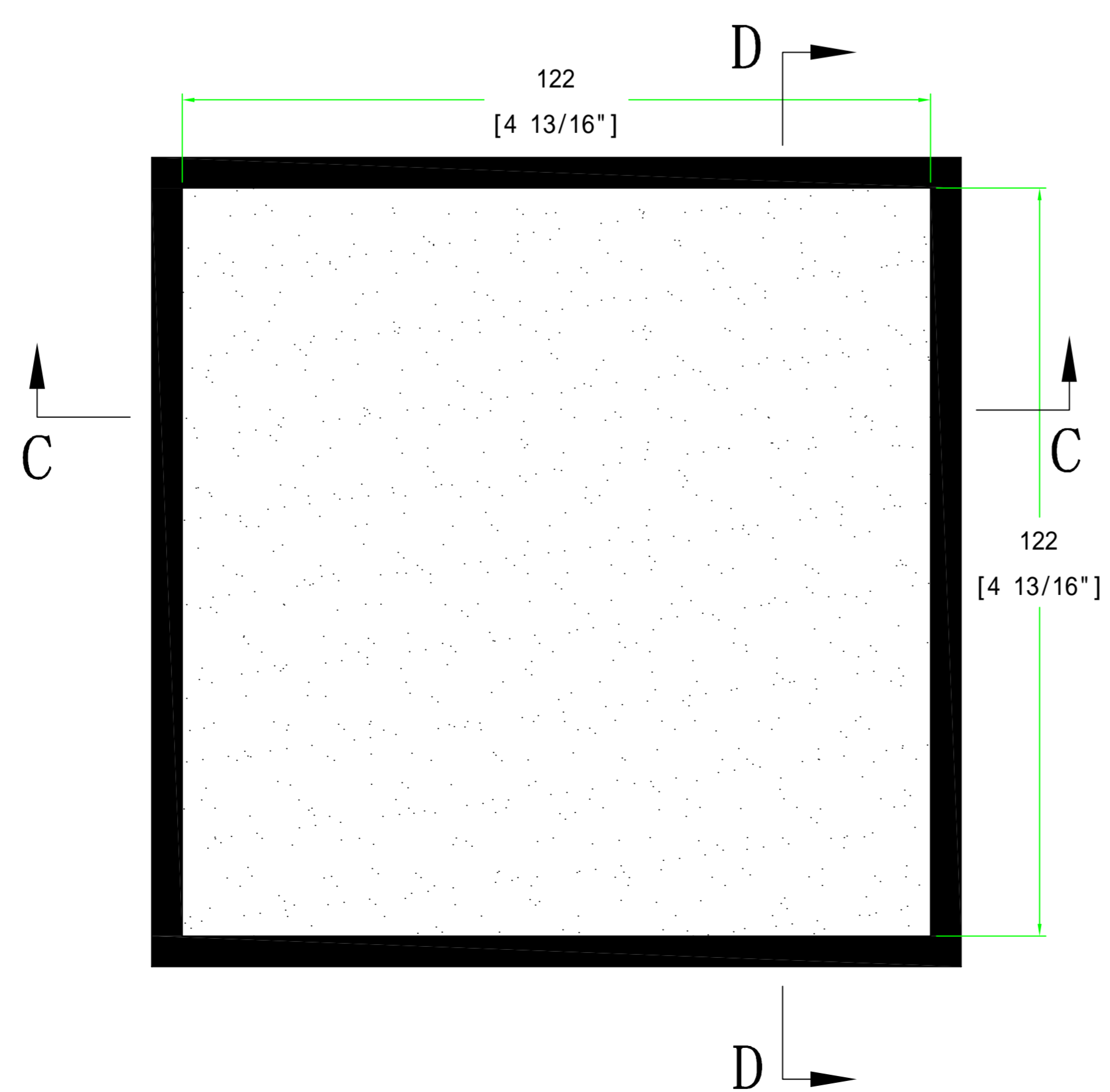
TOP VIEW OF BASE
