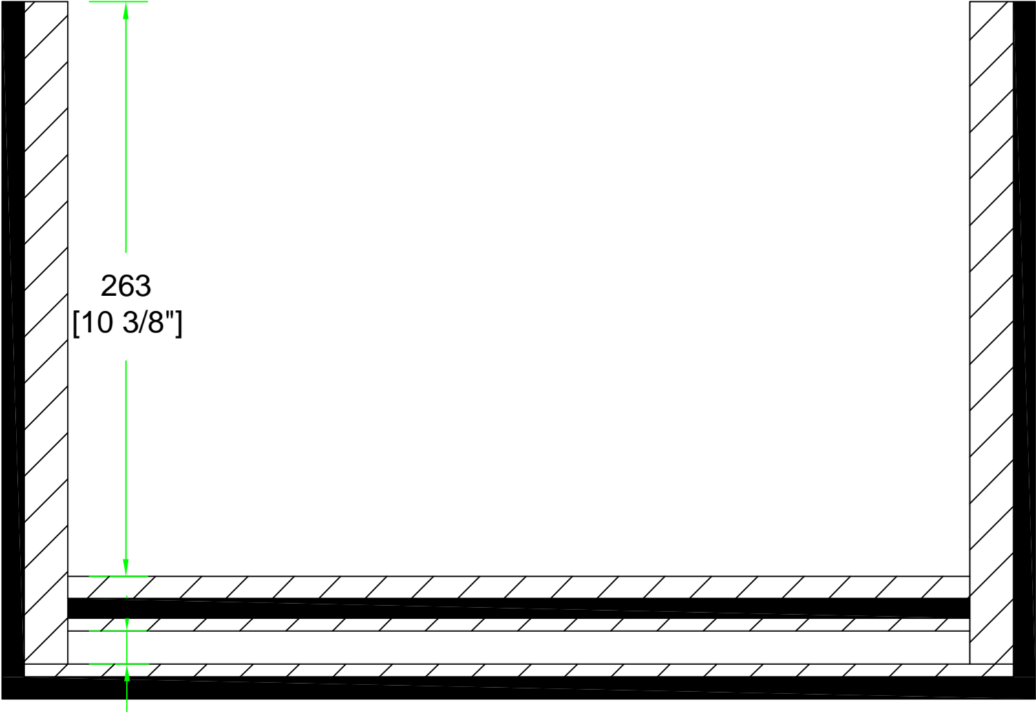
C-C VIEW
