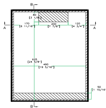
TOP VIEW OF BASE
