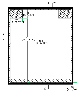
TOP VIEW OF COVER
