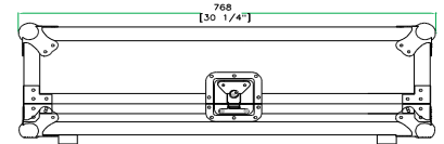
RIGHT VIEW
