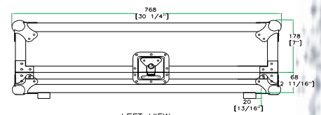
LEFT VIEW
